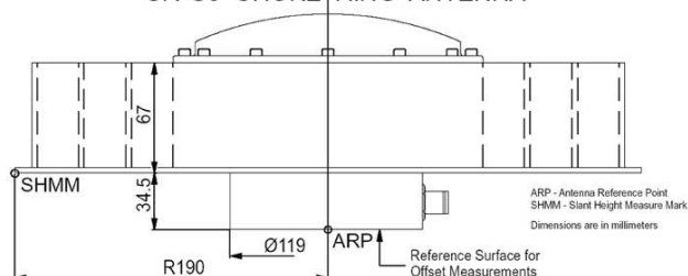
CR-G3 CHOKE RING ANTENNA
